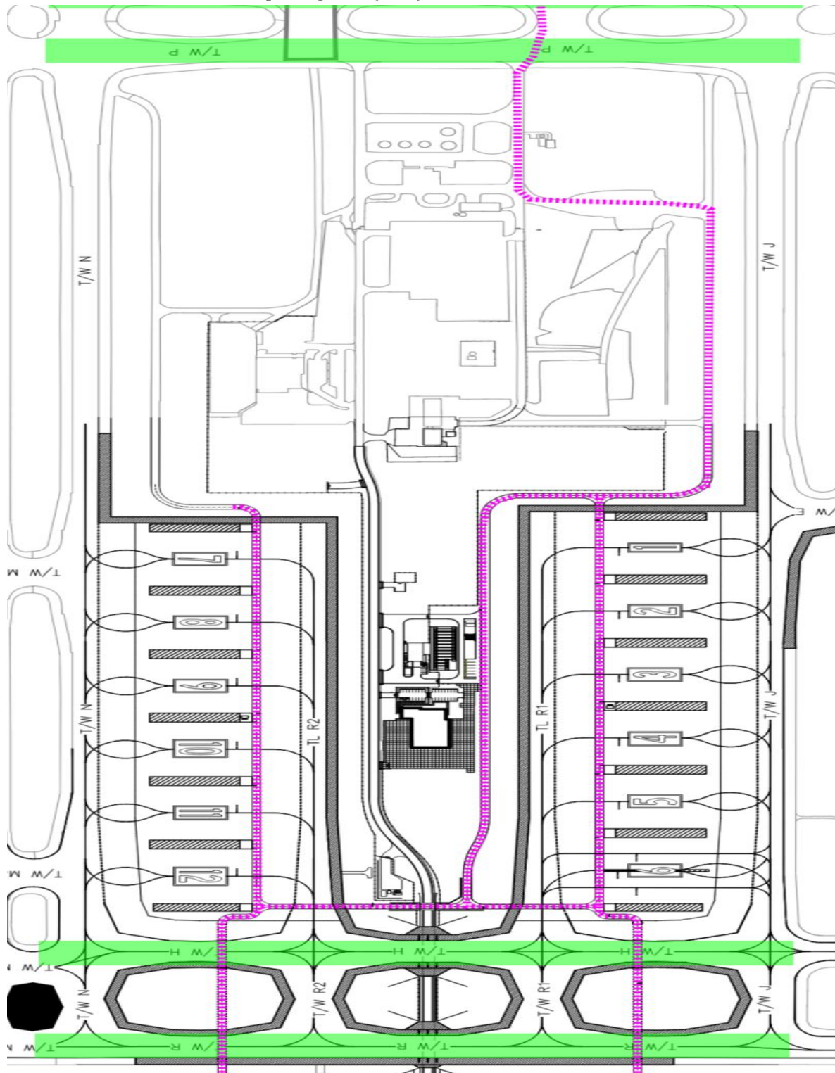
Figure 3 – MEM Centralized De-Icing Facility
